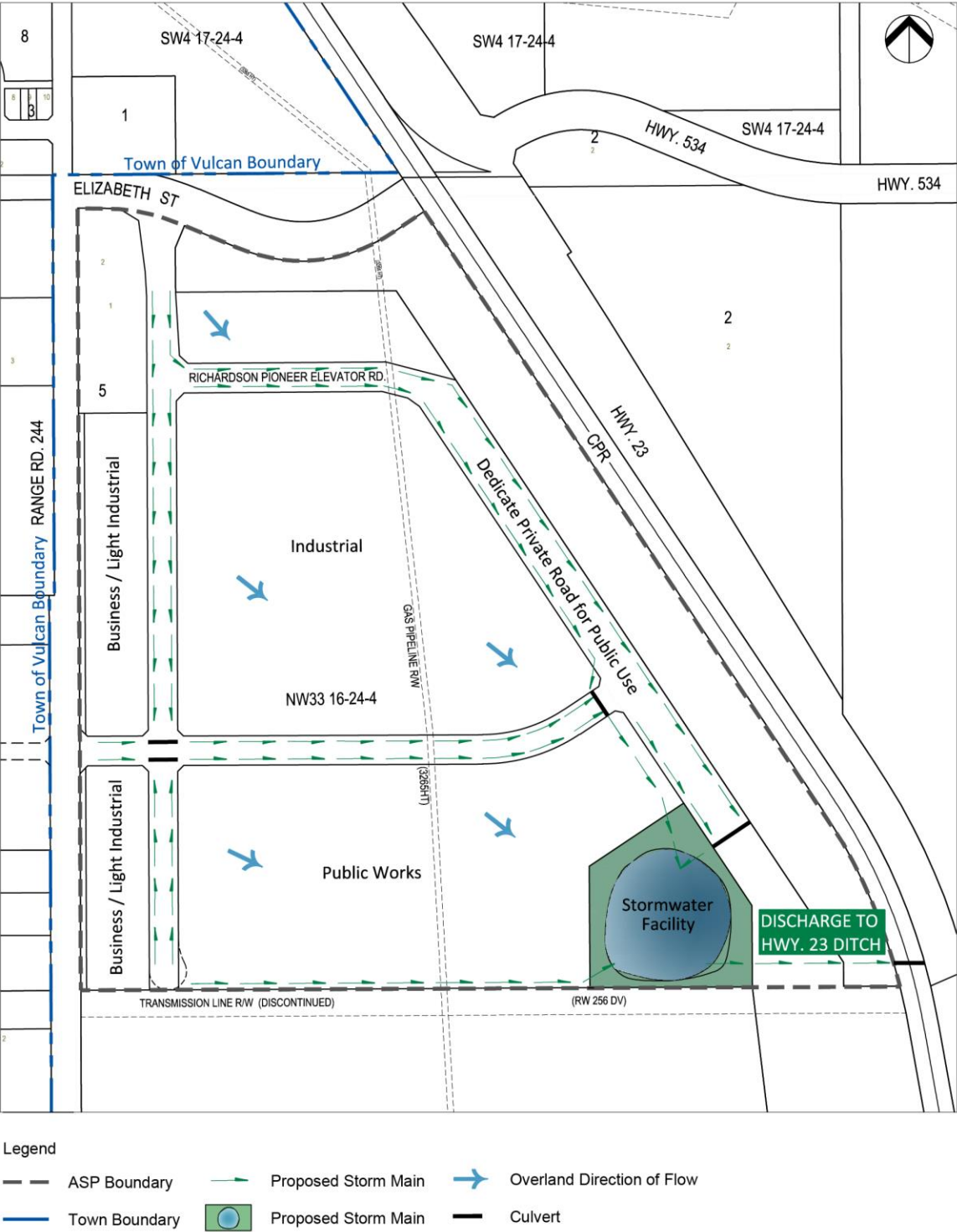
Figure 9 - Stormwater Servicing Plan
